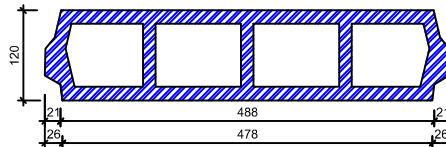
Block (530x200x120)
